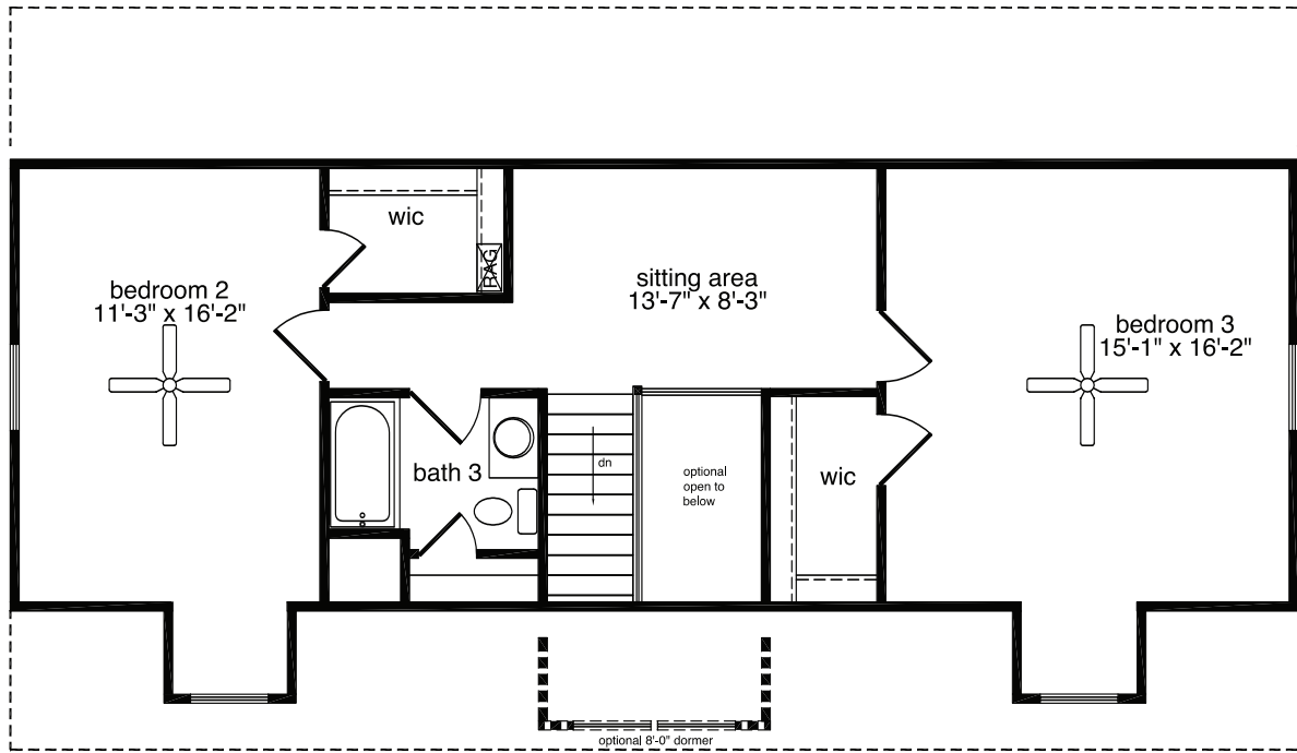
suggested second floor
